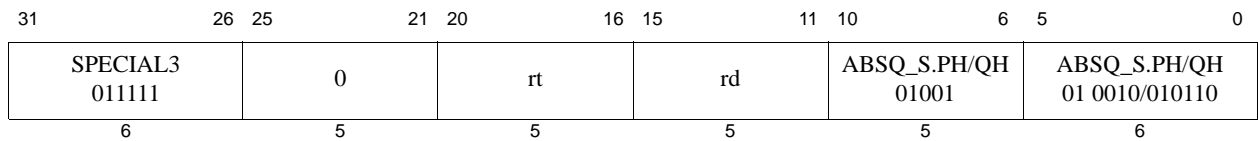
Figure 5.3 SPECIAL3 Encoding of ABSQ_S.PH/ABSQ_S.QH Instruction Sub-class without Immediate Field
