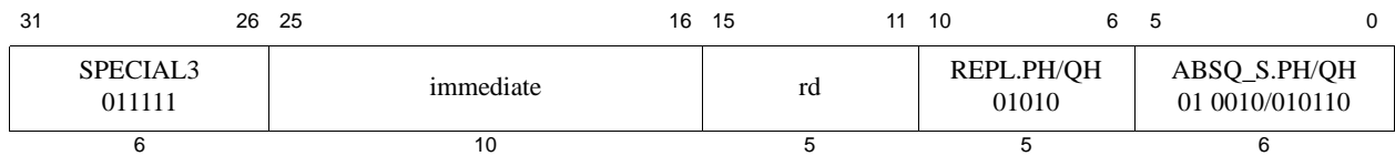
Figure 5.4 SPECIAL3 Encoding of ABSQ_S.PH/ABSQ_S.QH Instruction Sub-class with Immediate Field
